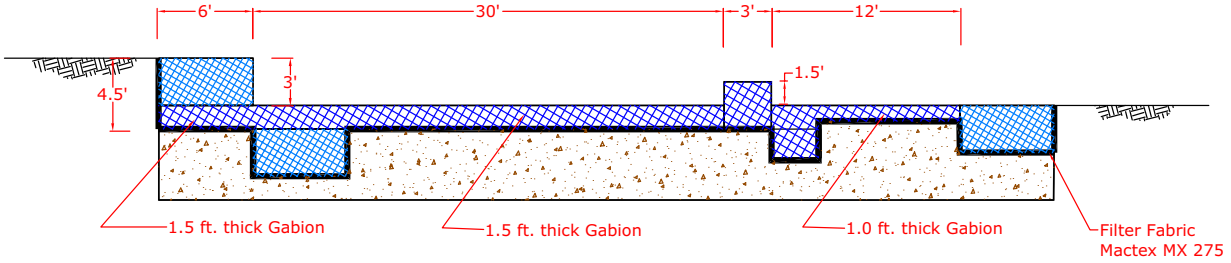
Typical long section through a drop structure
